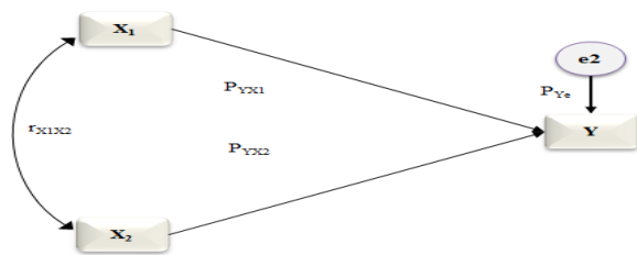
Gambar 1.1 Path Analysis
